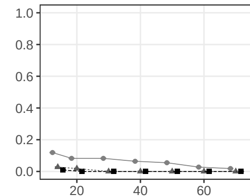
Proprtion of Negative ICCs
