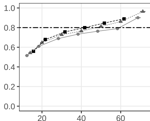
Correlation with Benchmark
